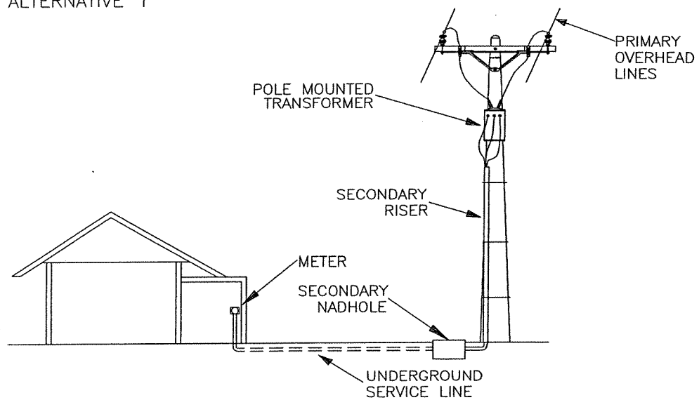
HYBRID DISTRIBUTION SYSTEM ALTERNATIVE 1
