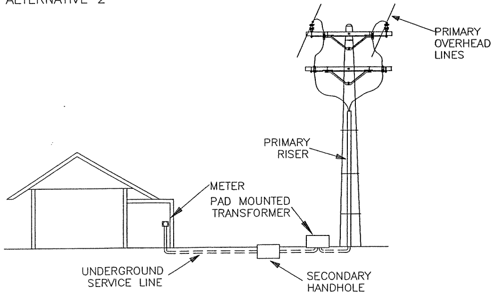
UNDERGROUND DISTRIBUTION SYSTEM ALTERNATIVE 2
